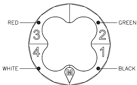
WIRE SIDE VIEW OF CONTACT HOLDER TO SHOW LABEL DETAILS
